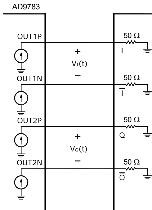
Figure 2. AD9783 Driving AM150175A
